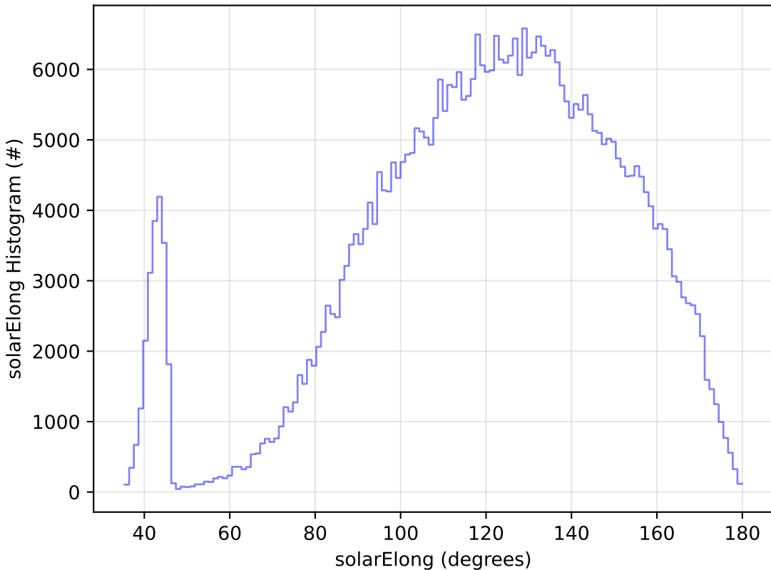
baseline_v3.5_10yrs All sky z band: solarElong Histogram
