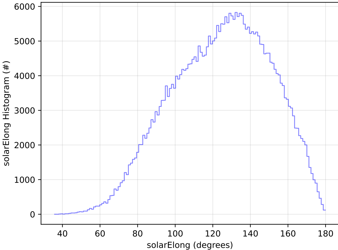
baseline_v3.5_10yrs All sky y band: solarElong Histogram
