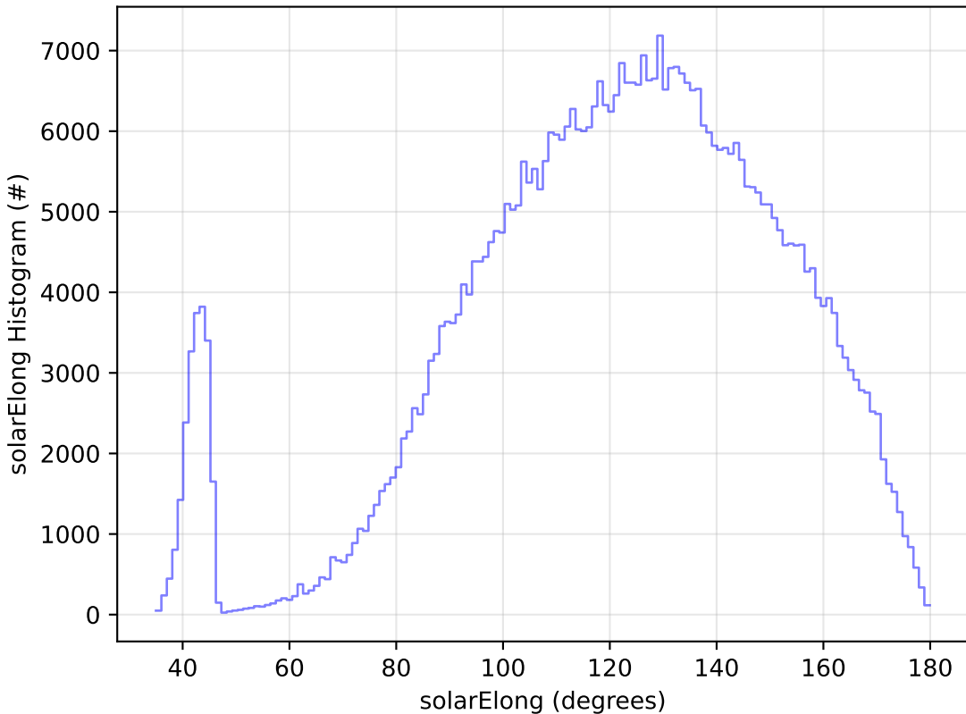
baseline_v3.5_10yrs All sky i band: solarElong Histogram
