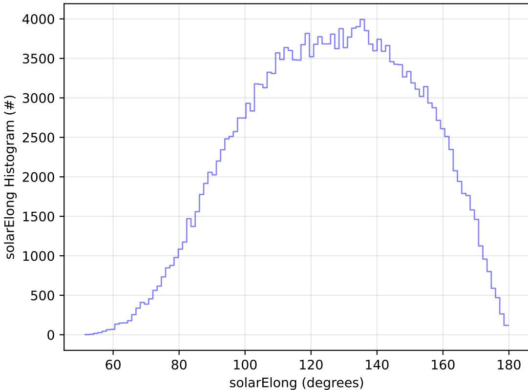
baseline_v3.5_10yrs All sky g band: solarElong Histogram
