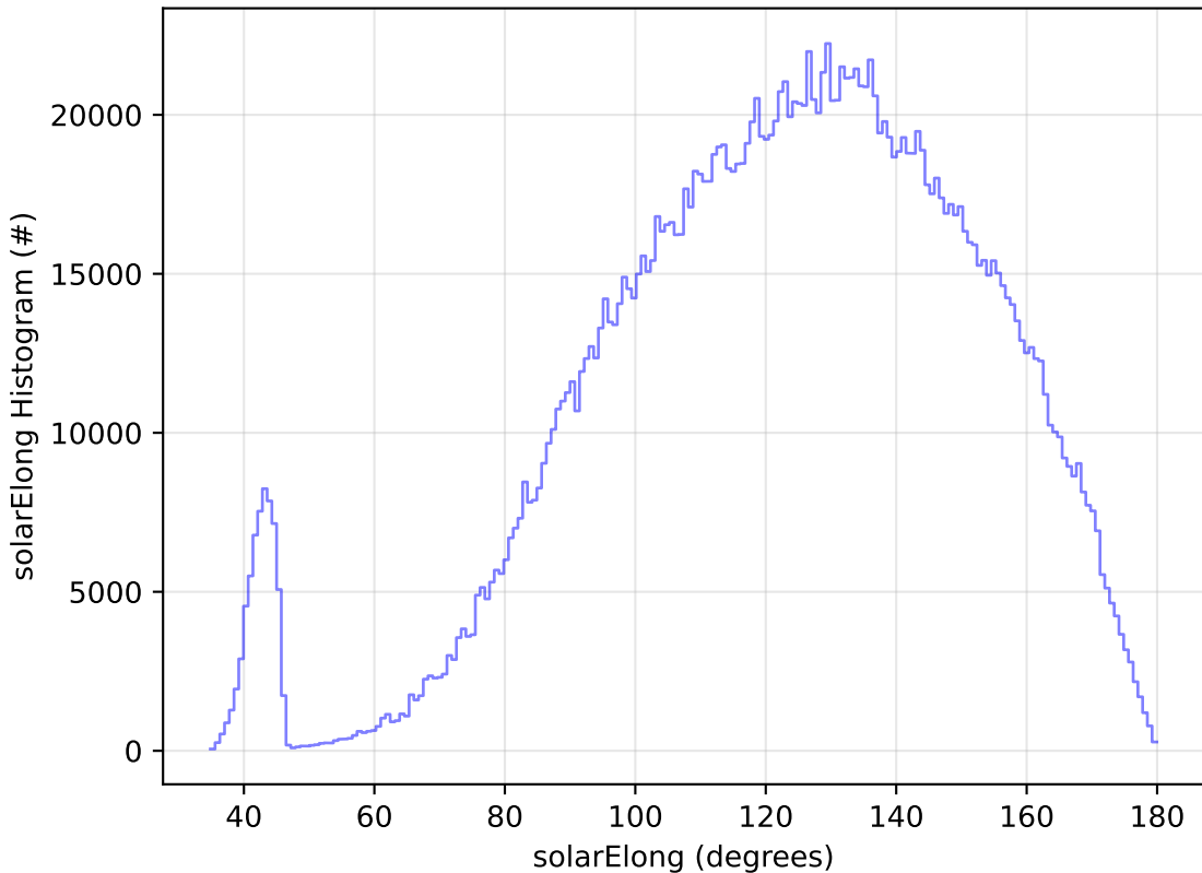
baseline_v3.5_10yrs All sky all bands: solarElong Histogram
