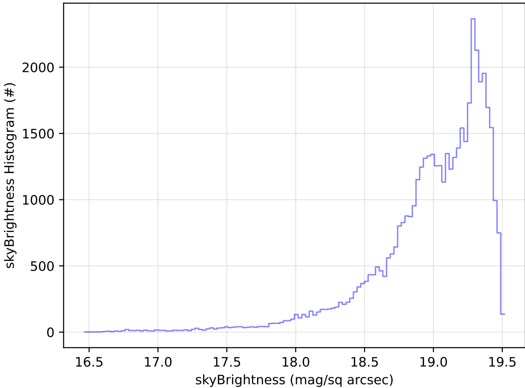
baseline_v3.5_10yrs Yr 1 z band: skyBrightness Histogram
