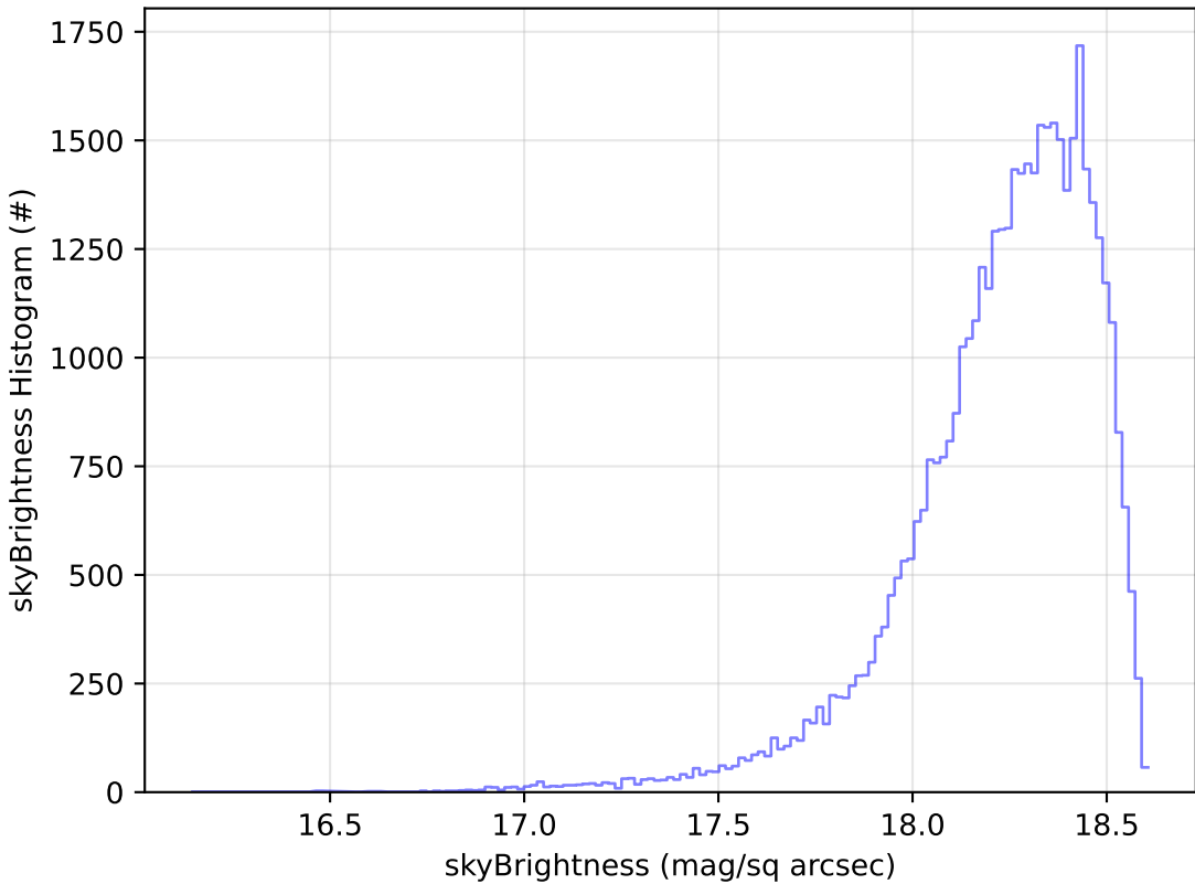
baseline_v3.5_10yrs Yr 1 y band: skyBrightness Histogram
