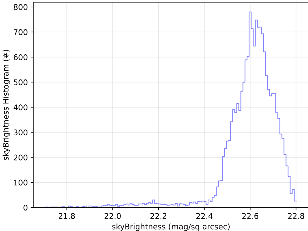
baseline_v3.5_10yrs Yr 1 u band: skyBrightness Histogram
