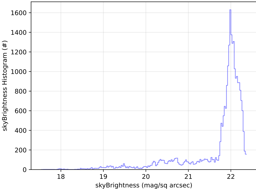
baseline_v3.5_10yrs Yr 1 g band: skyBrightness Histogram
