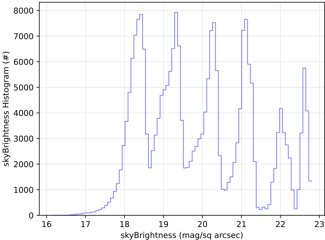
baseline_v3.5_10yrs Yr 1 all bands: skyBrightness Histogram
