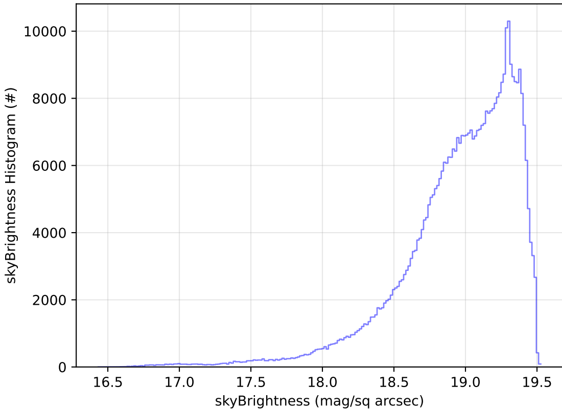
baseline_v3.5_10yrs WFD z band: skyBrightness Histogram
