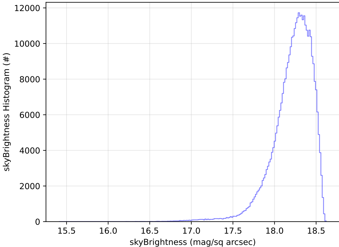
baseline_v3.5_10yrs WFD y band: skyBrightness Histogram
