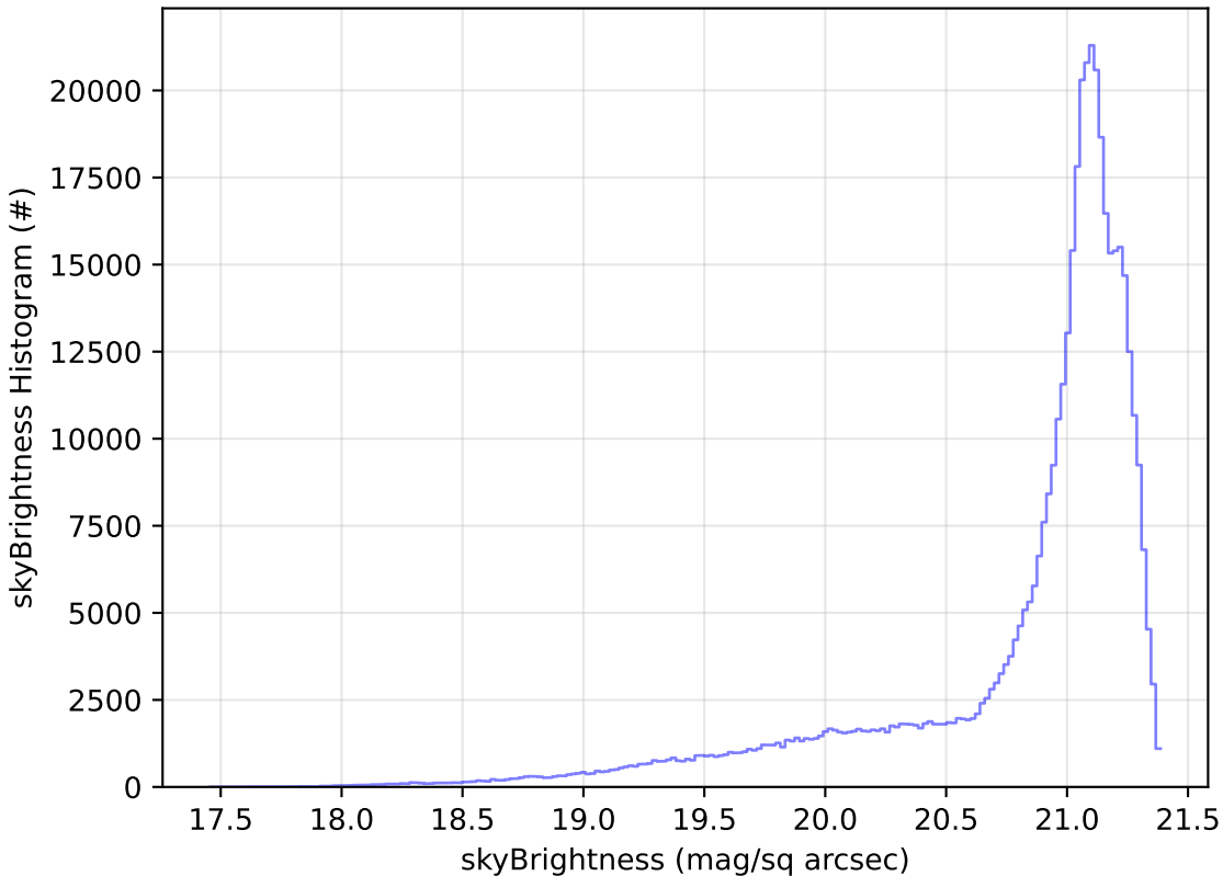
baseline_v3.5_10yrs WFD r band: skyBrightness Histogram
