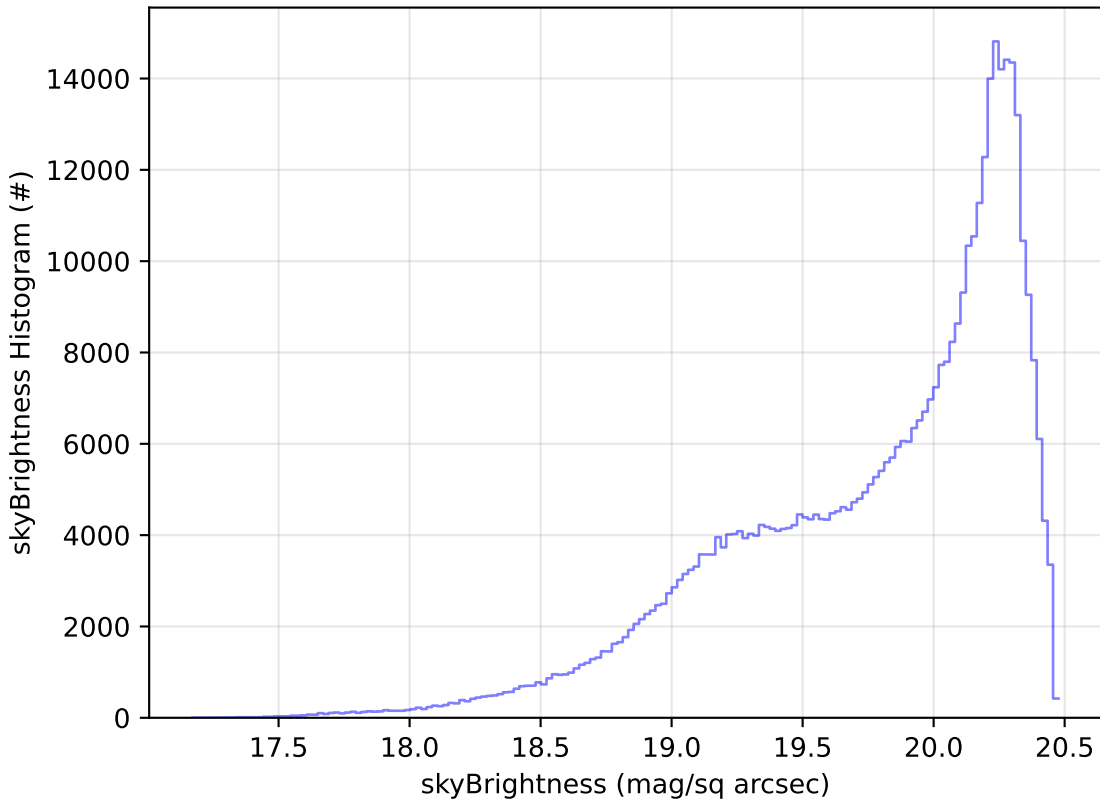
baseline_v3.5_10yrs WFD i band: skyBrightness Histogram
