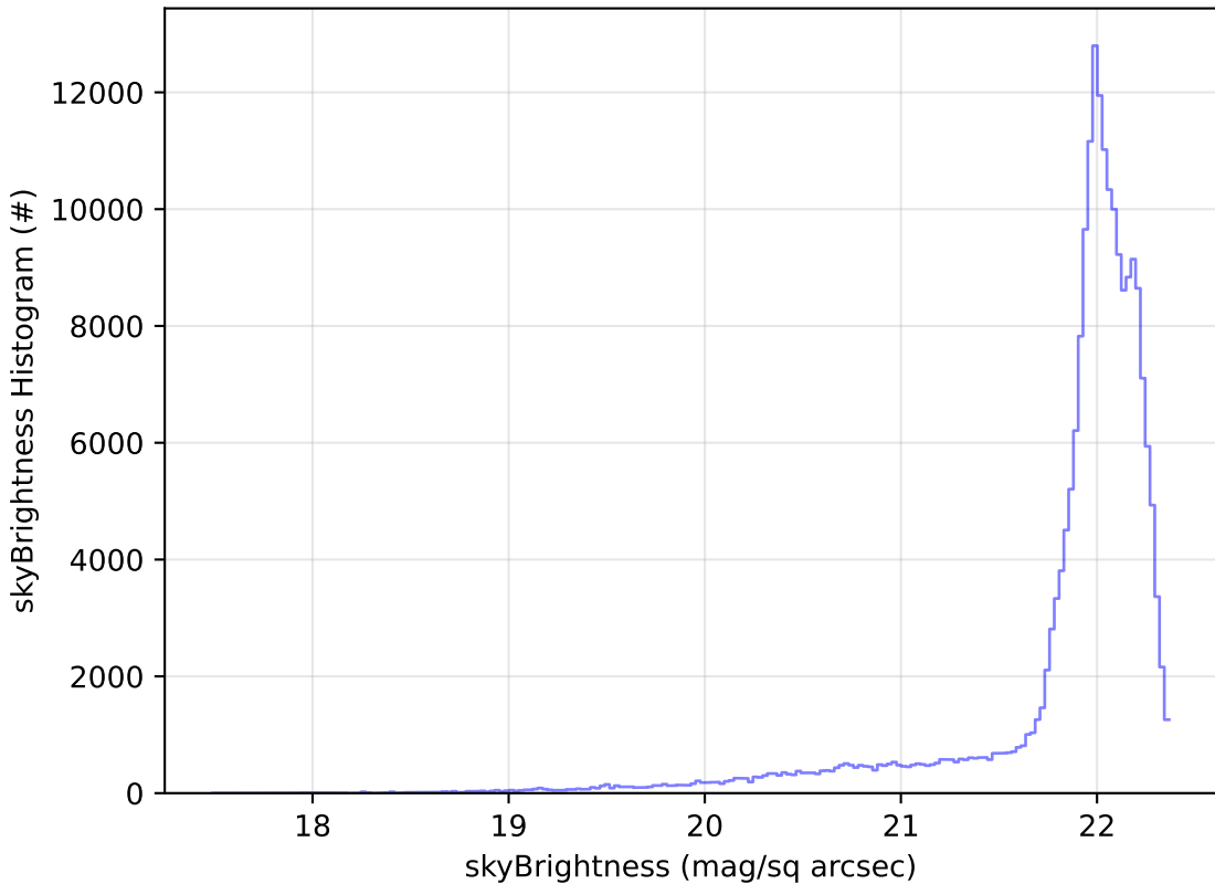
baseline_v3.5_10yrs WFD g band: skyBrightness Histogram
