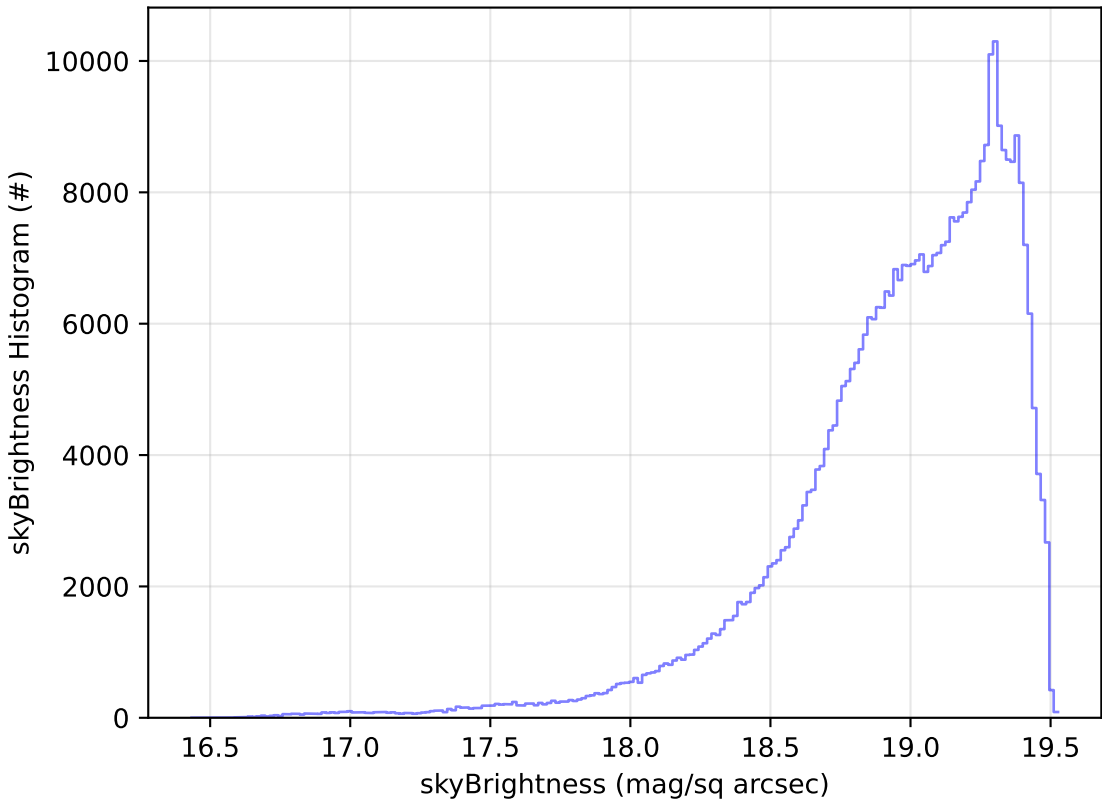
baseline_v3.5_10yrs All sky z band: skyBrightness Histogram
