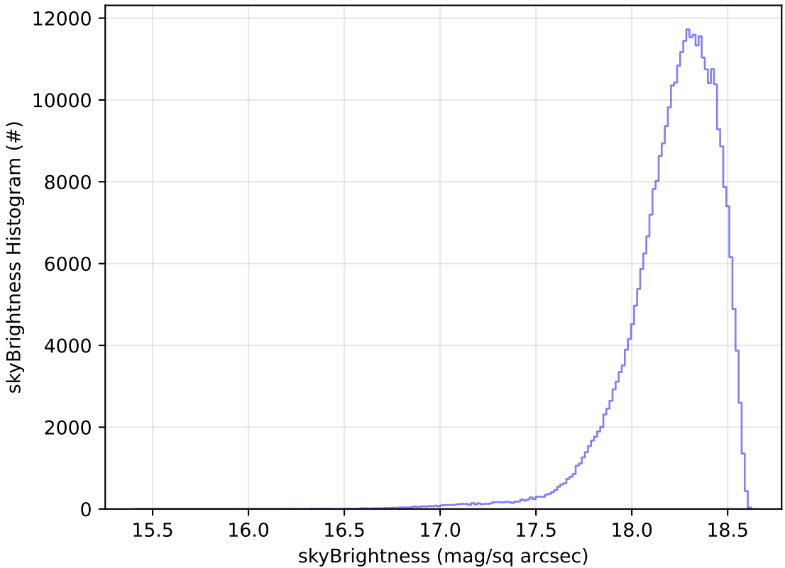
baseline_v3.5_10yrs All sky y band: skyBrightness Histogram
