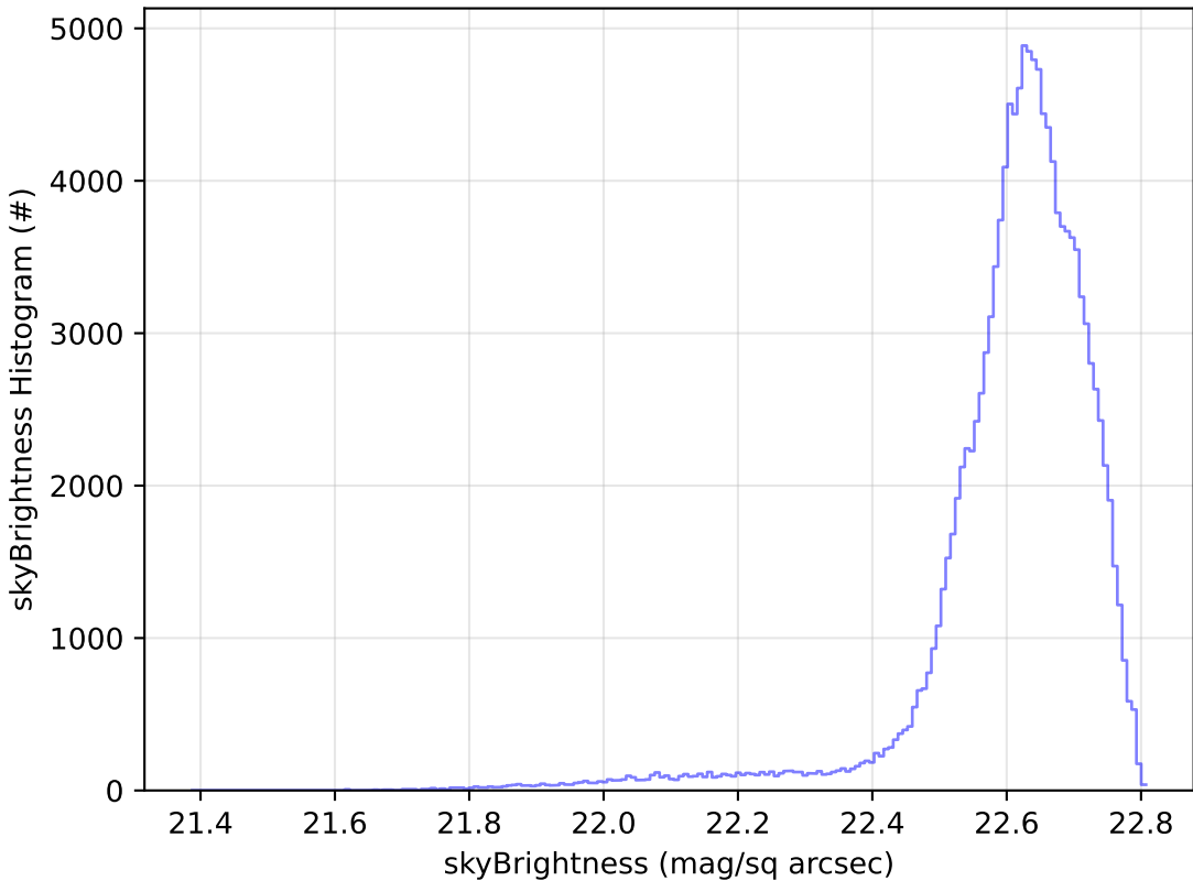
baseline_v3.5_10yrs All sky u band: skyBrightness Histogram
