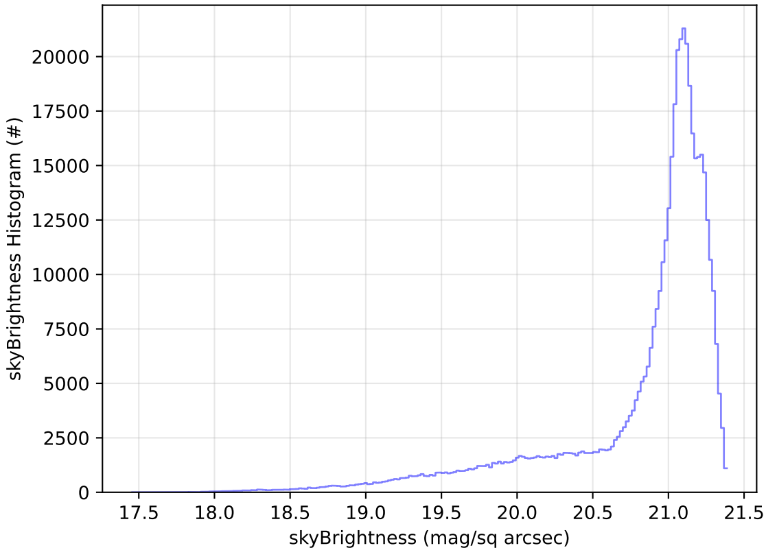
baseline_v3.5_10yrs All sky r band: skyBrightness Histogram
