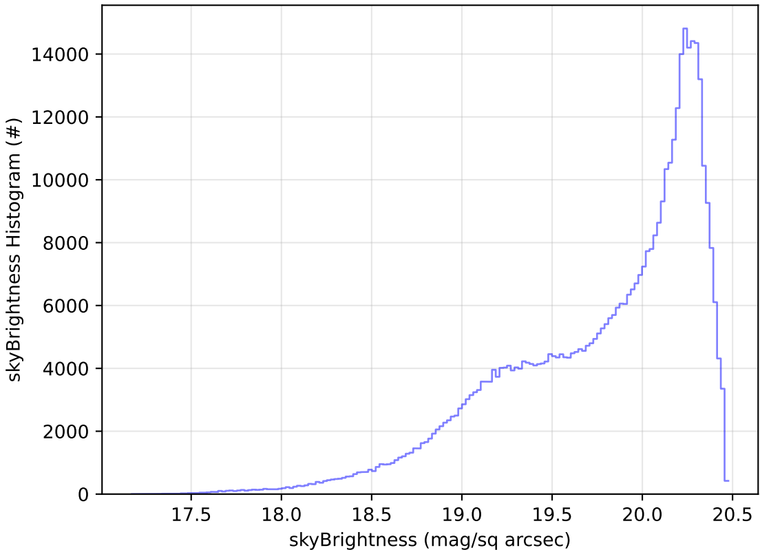
baseline_v3.5_10yrs All sky i band: skyBrightness Histogram
