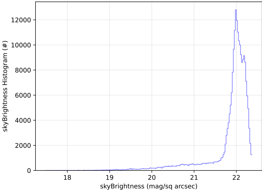
baseline_v3.5_10yrs All sky g band: skyBrightness Histogram
