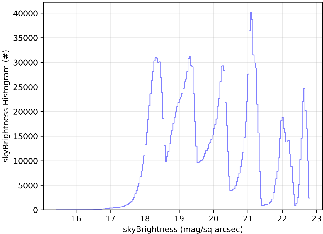
baseline_v3.5_10yrs All sky all bands: skyBrightness Histogram
