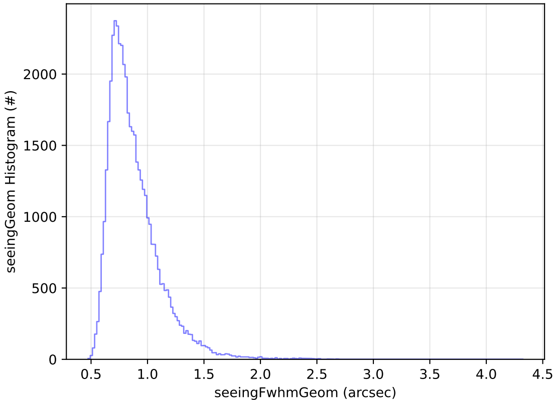
baseline_v3.5_10yrs Yr 1 z band: seeingGeom Histogram
