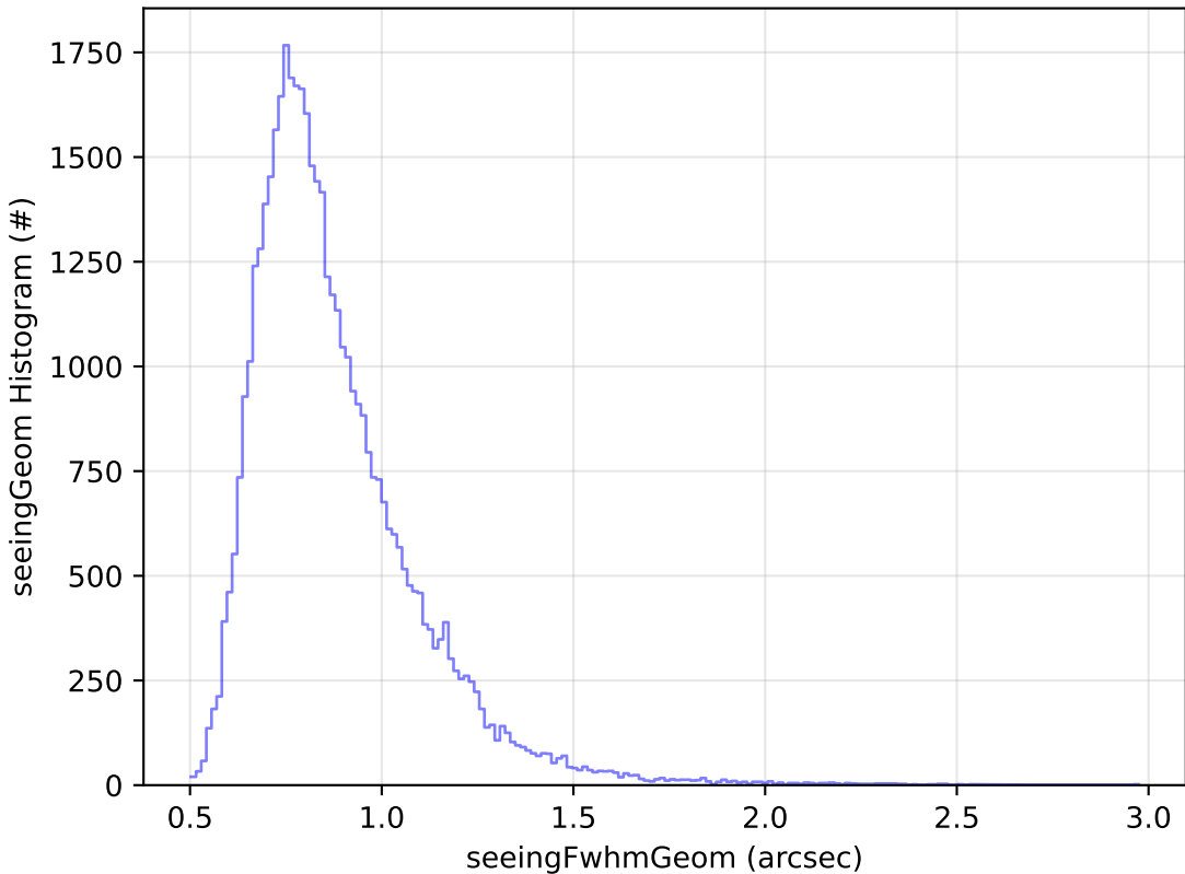
baseline_v3.5_10yrs Yr 1 y band: seeingGeom Histogram
