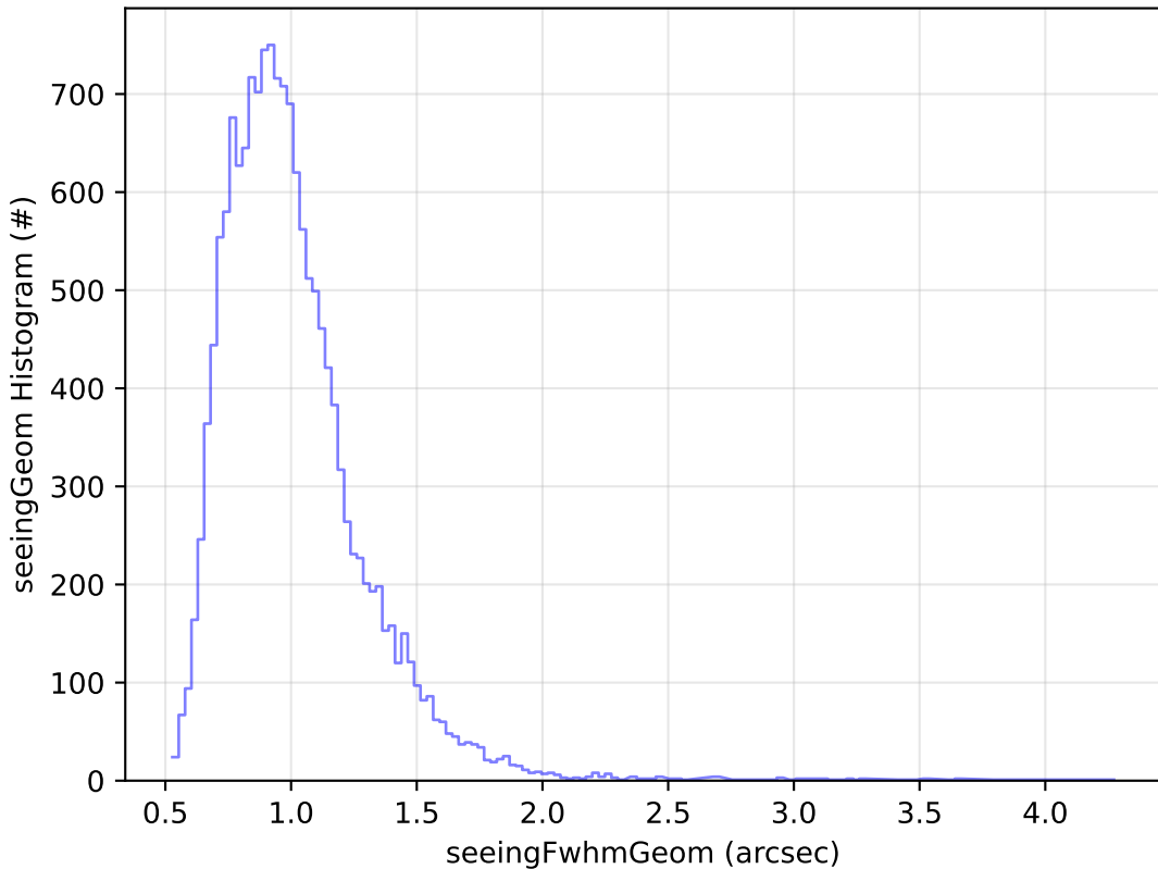
baseline_v3.5_10yrs Yr 1 u band: seeingGeom Histogram
