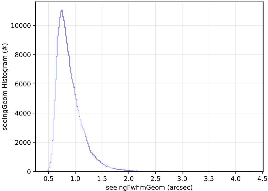
baseline_v3.5_10yrs Yr 1 all bands: seeingGeom Histogram
