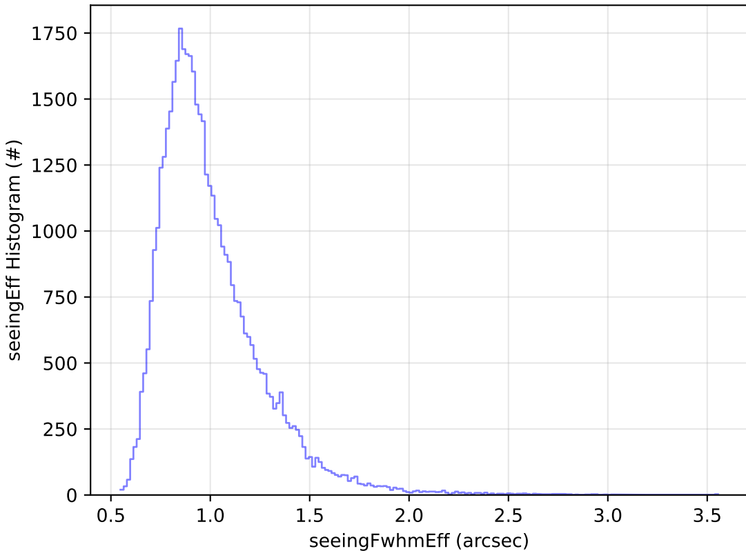
baseline_v3.5_10yrs Yr 1 y band: seeingEff Histogram
