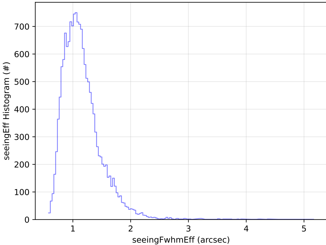
baseline_v3.5_10yrs Yr 1 u band: seeingEff Histogram
