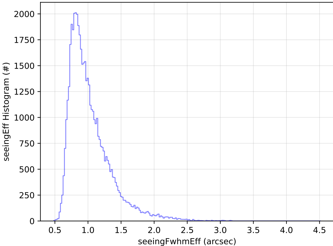
baseline_v3.5_10yrs Yr 1 r band: seeingEff Histogram
