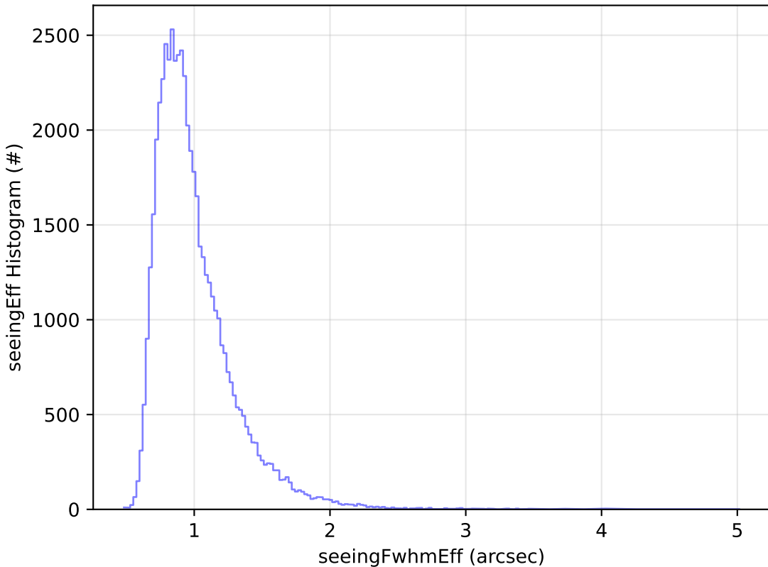
baseline_v3.5_10yrs Yr 1 i band: seeingEff Histogram
