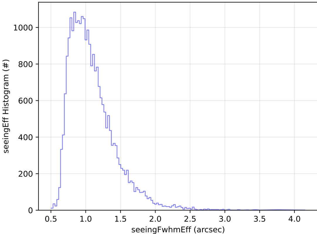
baseline_v3.5_10yrs Yr 1 g band: seeingEff Histogram
