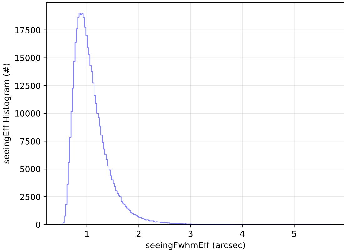
baseline_v3.5_10yrs WFD z band: seeingEff Histogram
