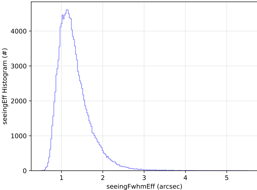
baseline_v3.5_10yrs WFD u band: seeingEff Histogram
