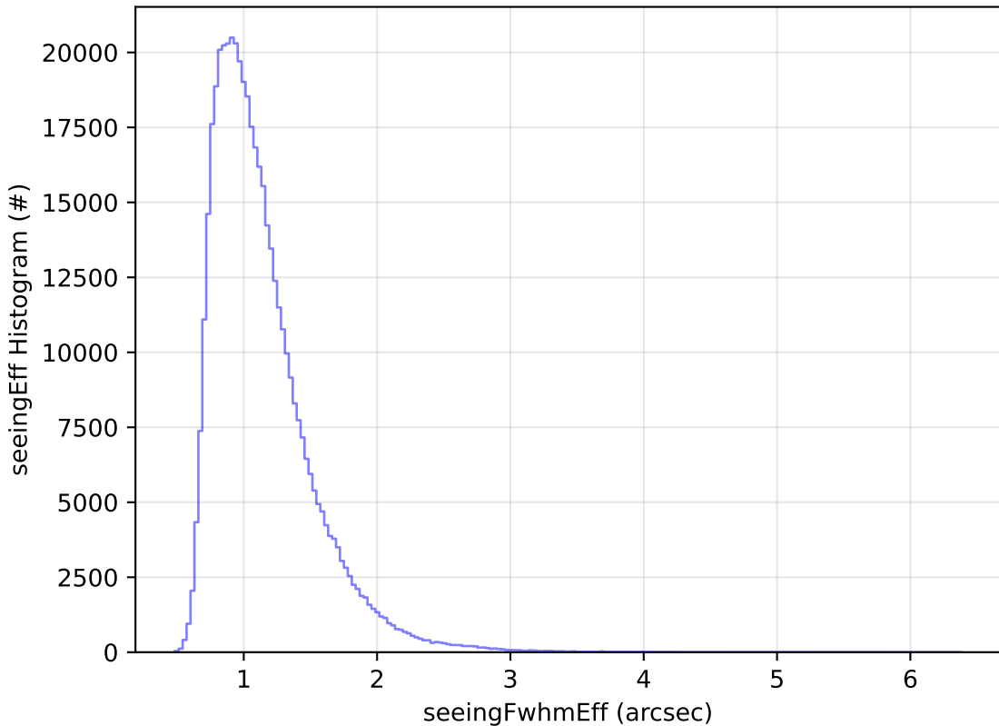
baseline_v3.5_10yrs WFD r band: seeingEff Histogram
