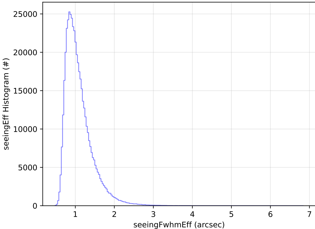
baseline_v3.5_10yrs WFD i band: seeingEff Histogram
