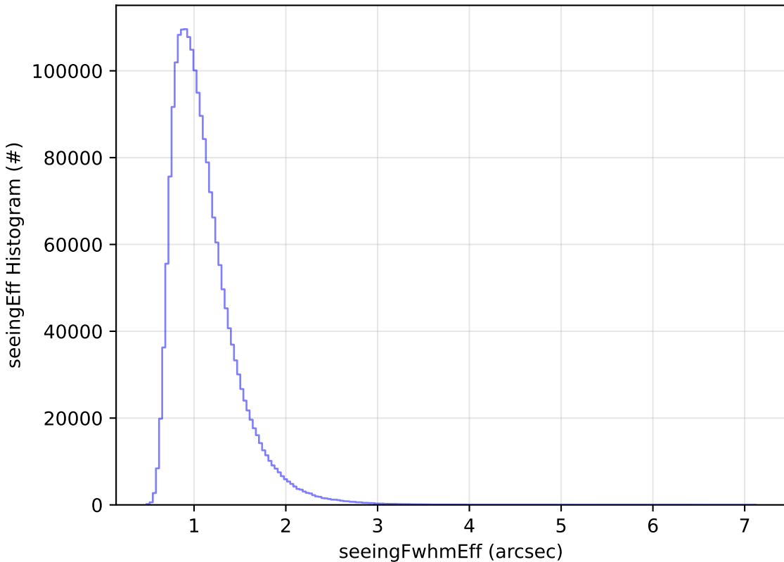
baseline_v3.5_10yrs WFD all bands: seeingEff Histogram
