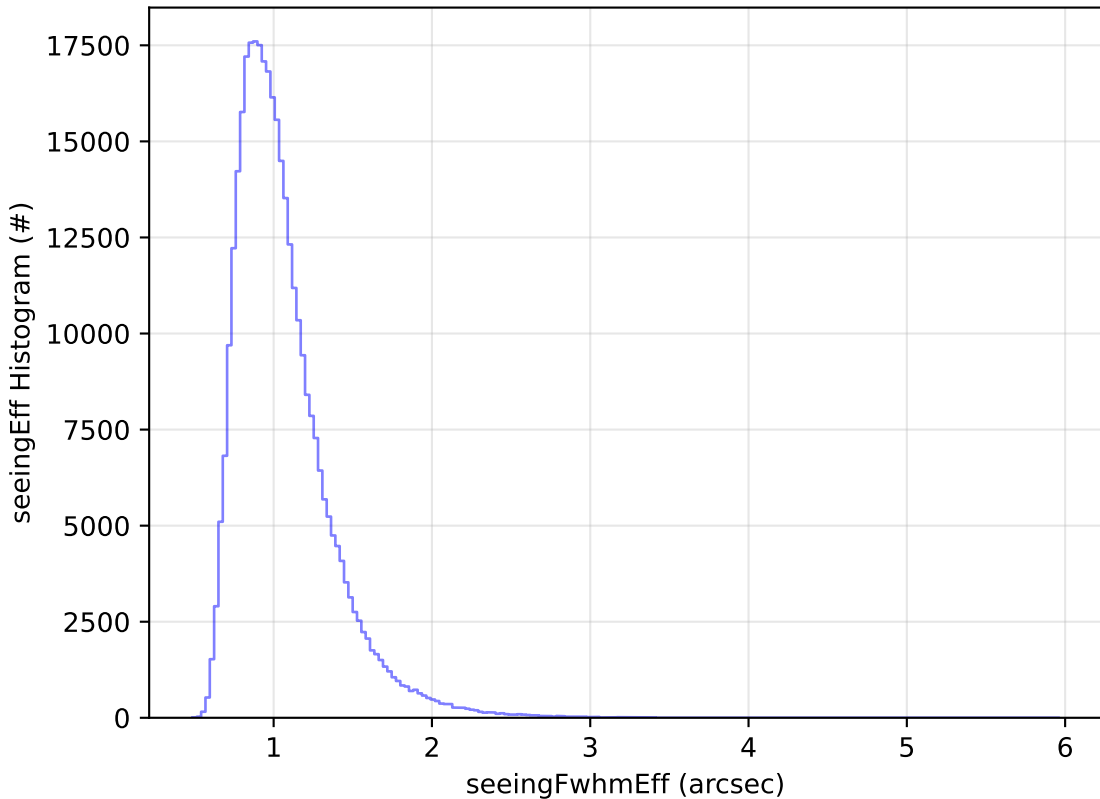
baseline_v3.5_10yrs All sky y band: seeingEff Histogram
