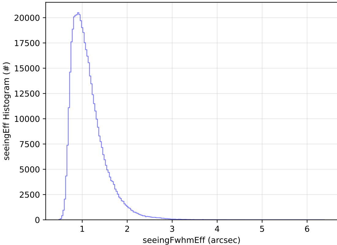
baseline_v3.5_10yrs All sky r band: seeingEff Histogram
