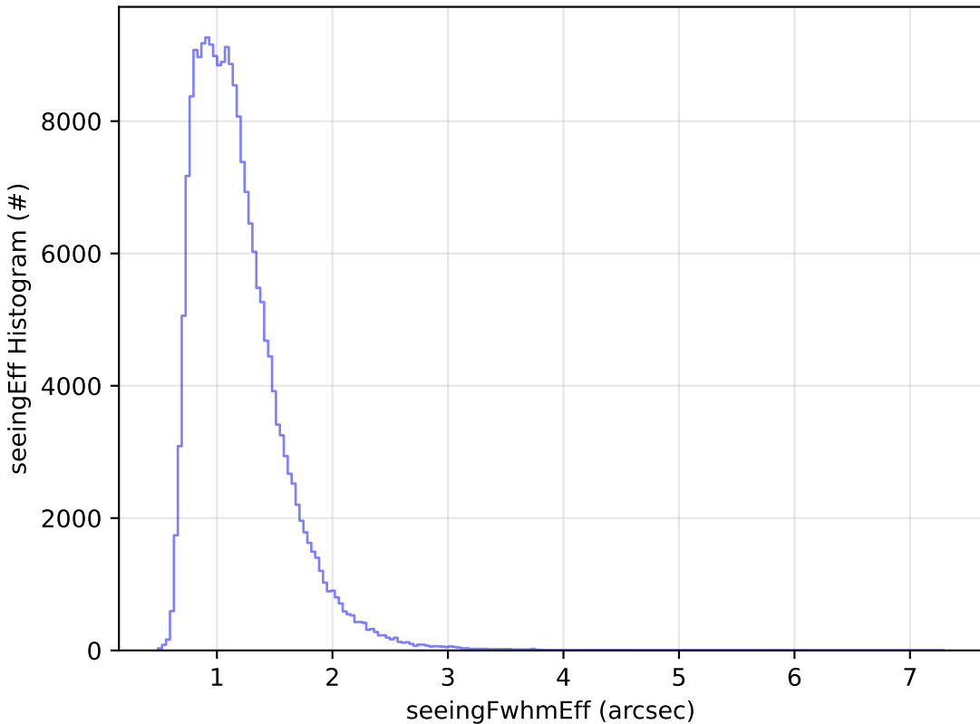
baseline_v3.5_10yrs All sky g band: seeingEff Histogram
