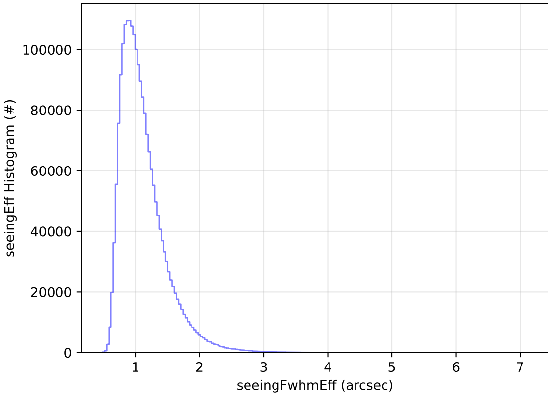
baseline_v3.5_10yrs All sky all bands: seeingEff Histogram
