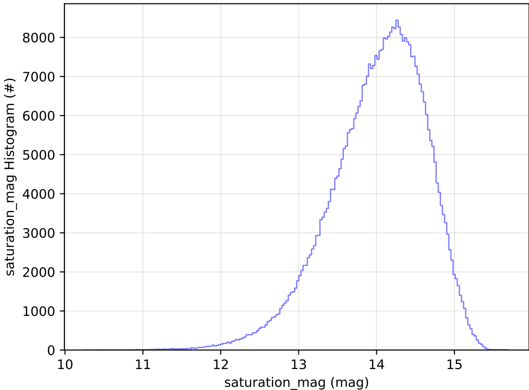
baseline_v3.5_10yrs WFD z band: saturation_mag Histogram
