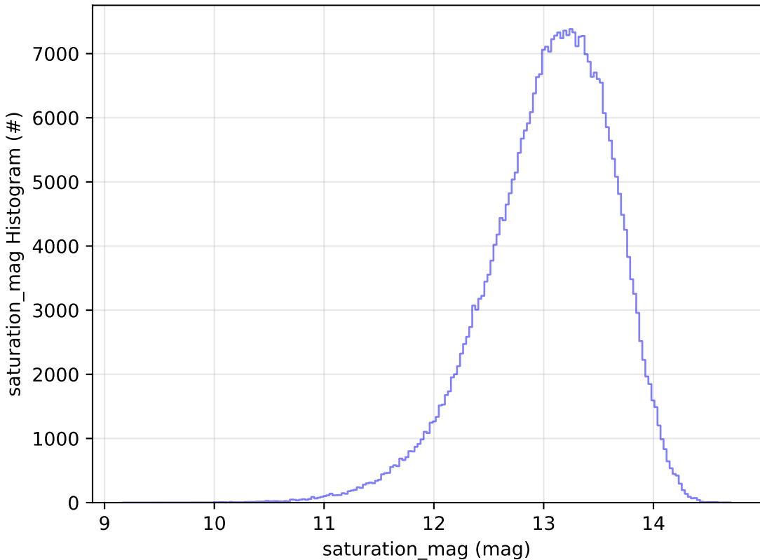
baseline_v3.5_10yrs WFD y band: saturation_mag Histogram
