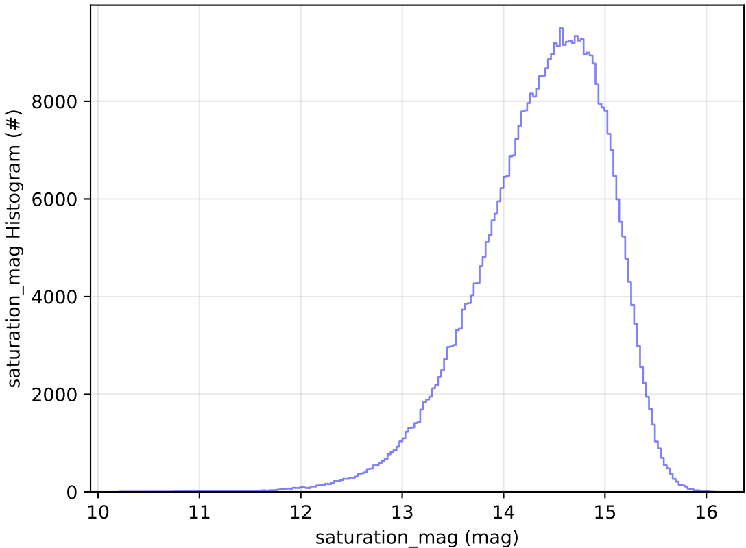
baseline_v3.5_10yrs WFD i band: saturation_mag Histogram
