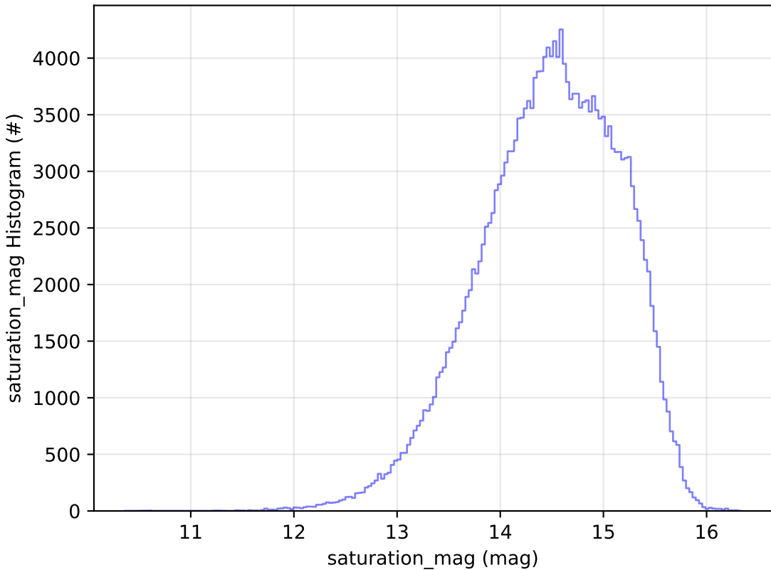
baseline_v3.5_10yrs WFD g band: saturation_mag Histogram
