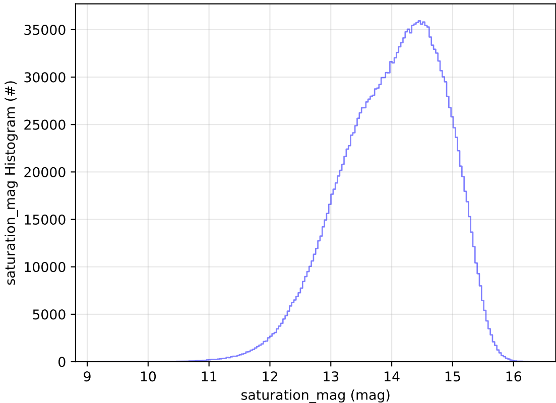
baseline_v3.5_10yrs WFD all bands: saturation_mag Histogram
