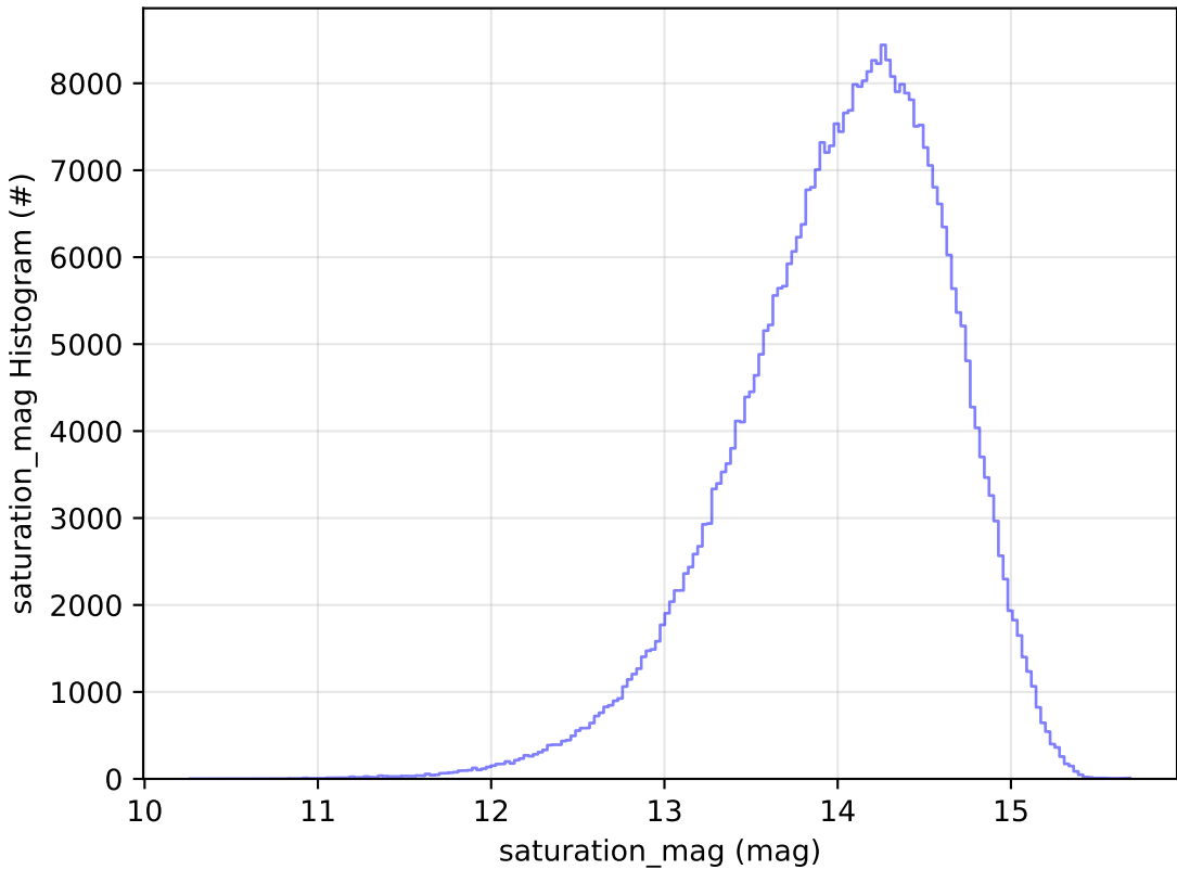
baseline_v3.5_10yrs All sky z band: saturation_mag Histogram
