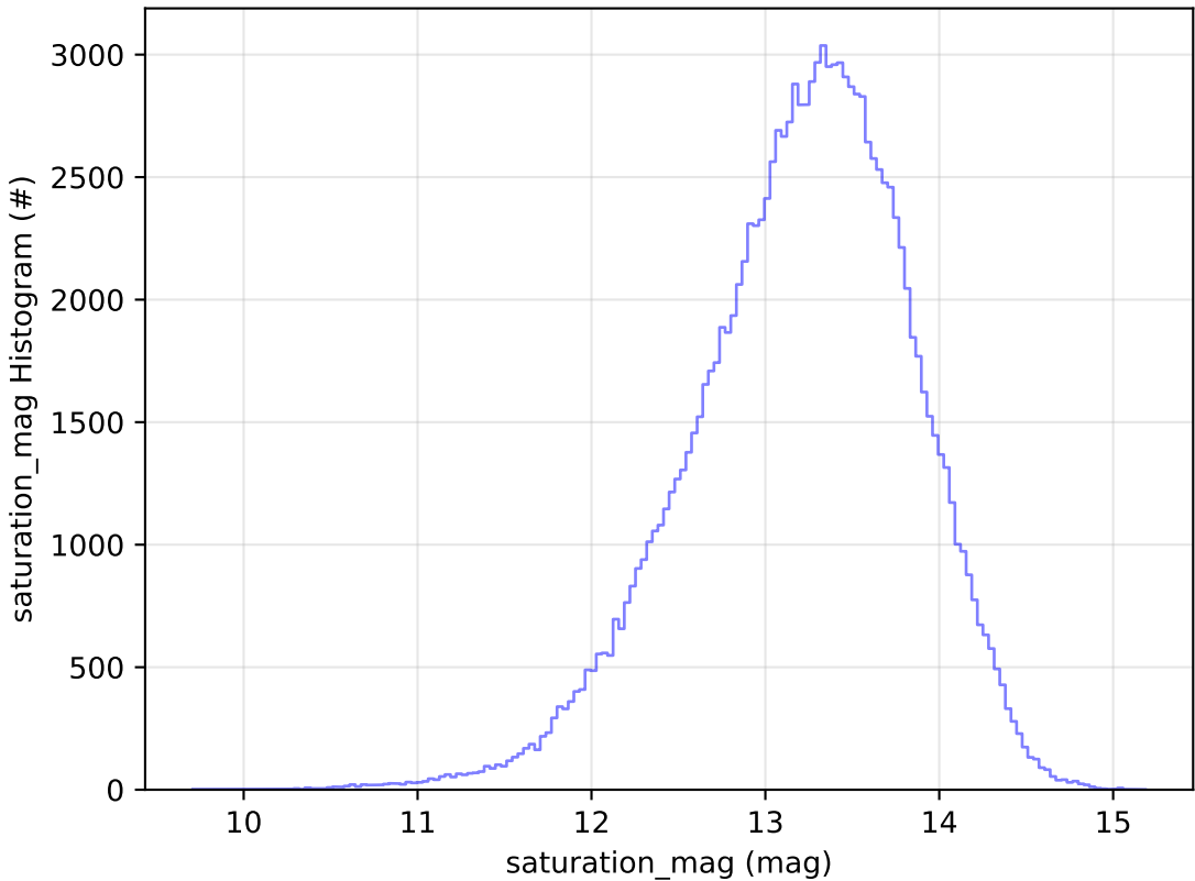
baseline_v3.5_10yrs All sky u band: saturation_mag Histogram
