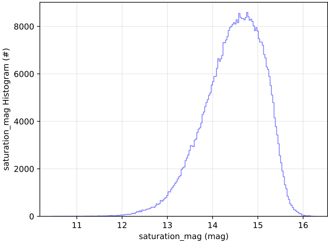
baseline_v3.5_10yrs All sky r band: saturation_mag Histogram
