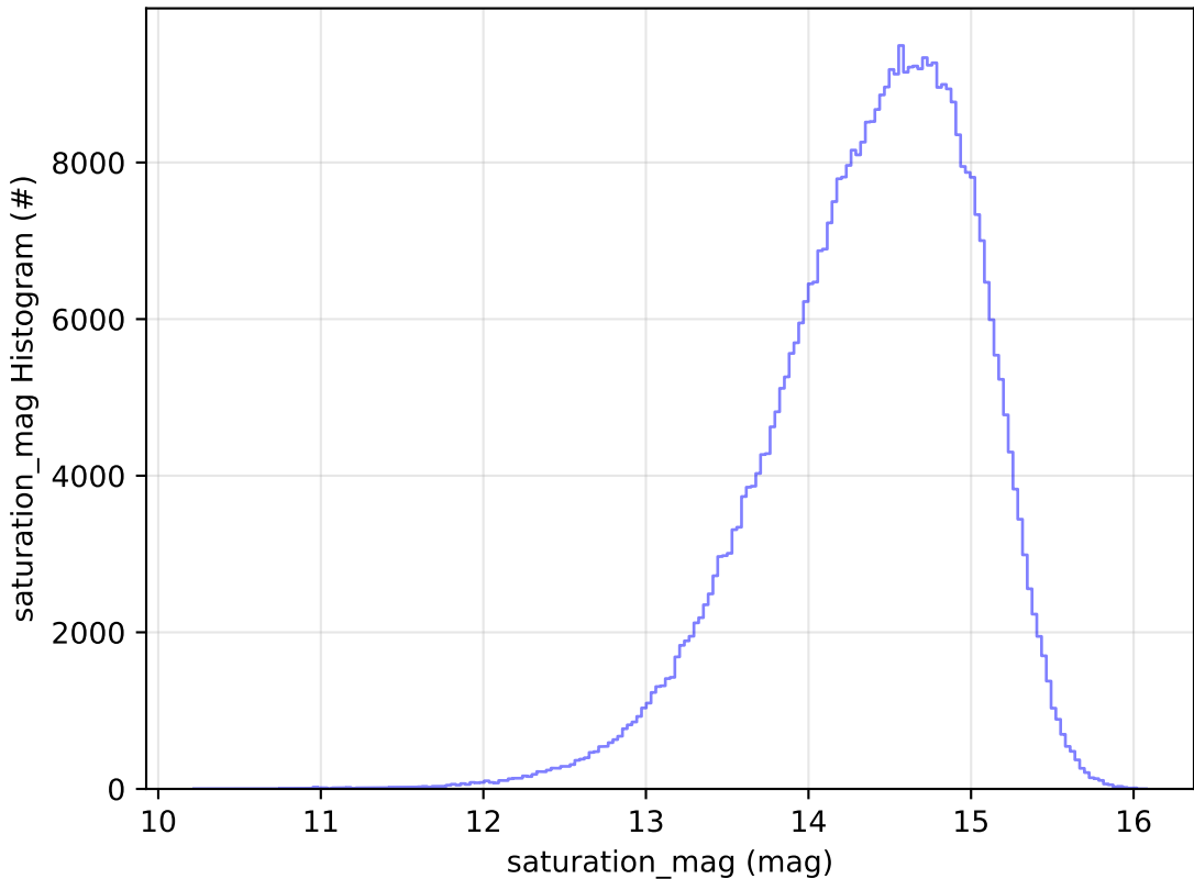
baseline_v3.5_10yrs All sky i band: saturation_mag Histogram
