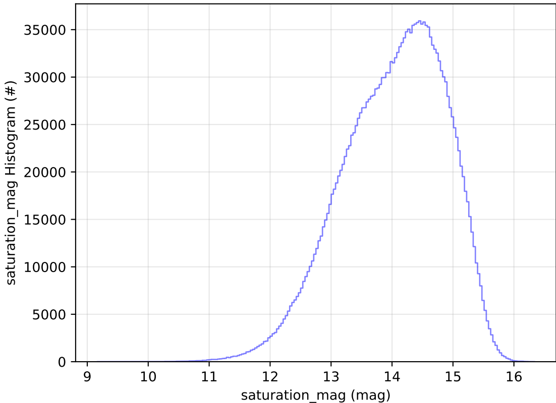
baseline_v3.5_10yrs All sky all bands: saturation_mag Histogram
